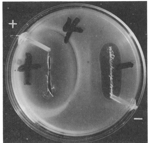
FIG. 3. Culture plate of S. aureus after 24 h of incubation with a 400- \mu A current and platinum electrodes. The bacteria were inhibited at both electrodes, but large pH shifts and gas formation were also encountered.
